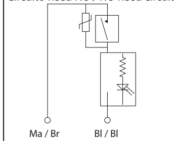
Circuito Reed NO / NO Reed Circuit
