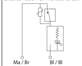
Circuito Reed NC / NC Reed Circuit
