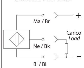
Circuito PNP / PNP Circuit
